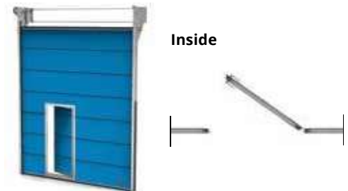
4. Hinge right / opening to the inside
